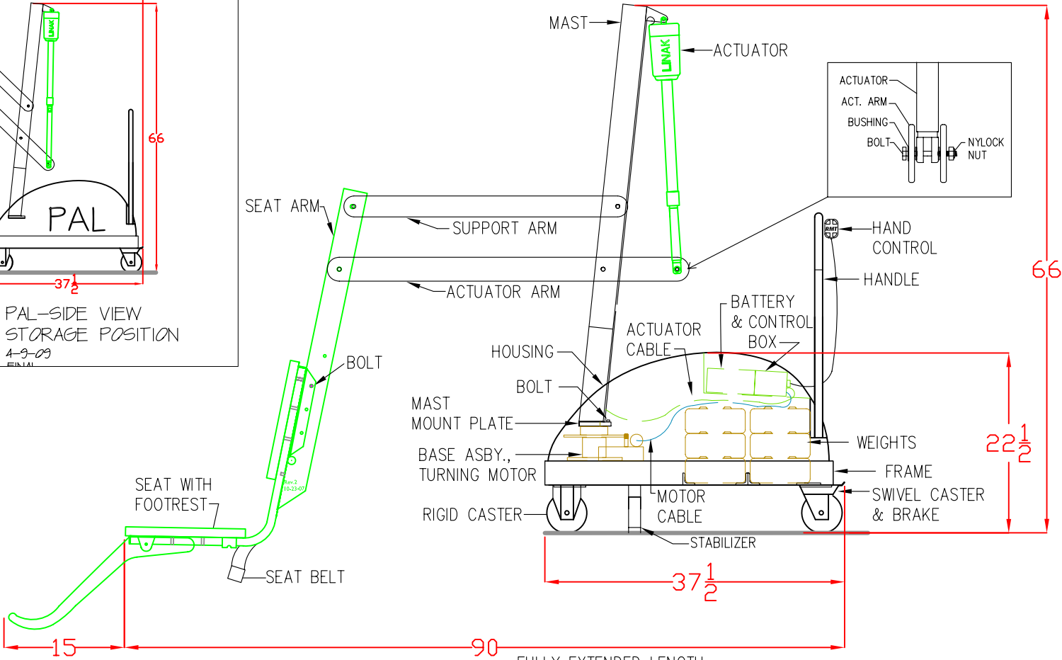
PAL-SIDE VIEW COMPONENT IDENTIFICATION 4-9-09 FINAL
